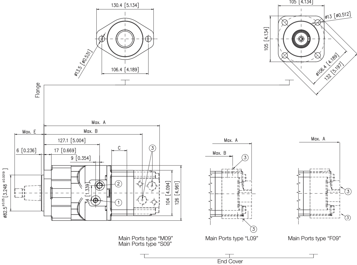
Type "A2" – SAE A 2 Bolts
